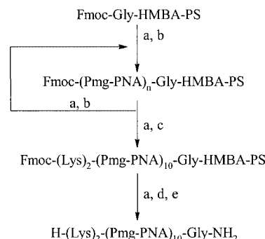
Scheme 7. Synthesis of all-( R )-Pmg PNA decamer IX ; reagents: (a) 22% piperidine/NMP (v/v); (b) Fmoc-Pmg-PNA building block 18a–c , DIEA, HBTU, 2×17.5 min; (c) Fmoc-L-Lys(Boc)-OH, DIEA, HBTU, 2×17.5 min; (d) 95% aqueous TFA; (e) NH 3 /MeOH saturated, 16 h, 55 °C
