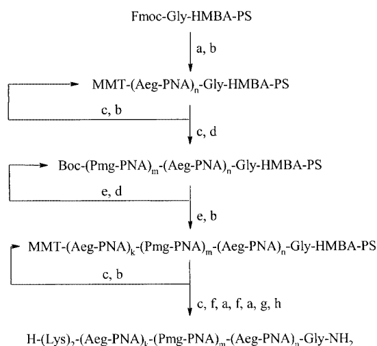
Scheme 5. Solid-phase synthesis of Pmg-PNA by a mixed protecting group strategy; reagents: (a) 22% piperidine/NMP (v/v); (b) MMT-Aeg-PNA building block, DIEA, HBTU; (c) 1% TFA/dichloroethane (v/v); (d) Boc-Pmg-PNA building block 1a or 1b , DIEA, HBTU; (e) TFA/DCM 1:1 (v/v); (f) Fmoc-L-Lys(Boc)-OH, DIEA, HBTU; (g) 95% aq. TFA; (h) NH 3 /MeOH saturated, 16 h, 55 °C
