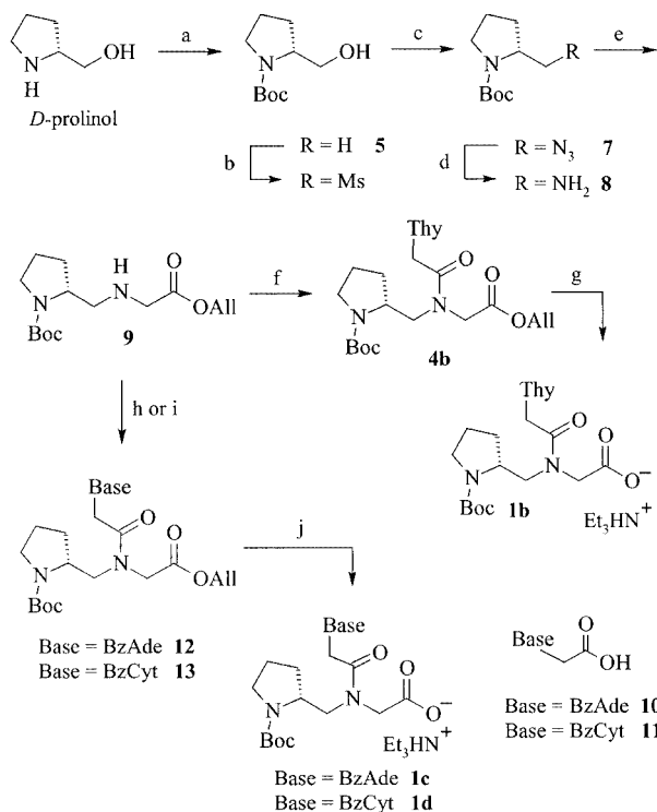
Scheme 2. Synthesis of adenine, cytosine and thymine ( R )-Pmg monomers; reagents: (a) Boc 2 O, 1 M NaOH (aq.), dioxane; (b) MsCl, Et 3 N, THF; (c) LiN 3 , DMF, 16 h, 64 °C; (d) Ph 3 P, H 2 O, THF; (e) BrCH 2 COOAllyl, Et 3 N, THF; (f) 3 , DIEA, HBTU, DMF; (g) 1) 2 M NaOH (aq.) dioxane, 2) KHSO 4 (pH 2), 3) Et 3 N; (h) 10 , DIEA, HBTU, DMF; (i) 11 , DIEA, HBTU, DMF (j) Bu 3 SnH, [Pd(PPh 3 ) 2 ]Cl 2 , AcOH, CH 2 Cl 2 , 10 min
