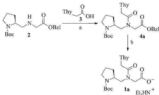
Scheme 1. Synthesis of thymine ( S )-Pmg monomer; reagents: (a) HBTU, DIEA, DMF, DMAP; (b) 1) 2 M NaOH, dioxane, 2) KHSO 4 (pH 2.0), 3) Et 3 N
