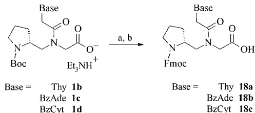
Scheme 6. Synthesis of Fmoc ( R )-Pmg monomers; reagents: (a) TFA/DCM/MeOH/H 2 O 16:16:1:1 (v/v/v/v); (b) FmocOSu, DIEA, THF
