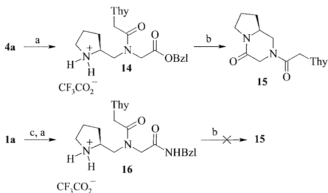
Scheme 3. Reagents: (a) 50% TFA/CH 2 Cl 2 ; (b) 15 equiv. DIEA as 0.4 M solution in DMF; (c) BzNH 2 , HBTU, DIEA, DMF
