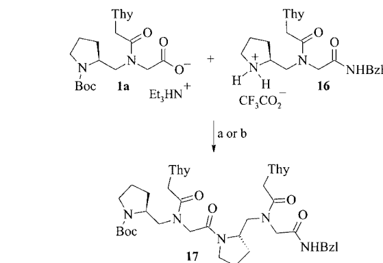
Scheme 4. Coupling in solution; reagents: (a) HBTU, DIEA, DMF; (b) PyBroP ® , DIEA, DMF
