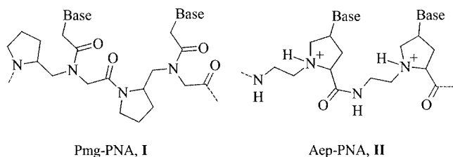
Figure 1. Structures of Pmg- and Aep-PNAs
